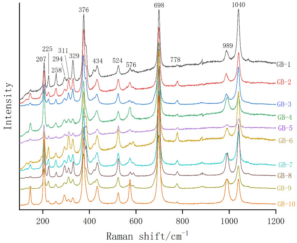
Raman spectra of all ten samples of jadeite matrix. Spectra are stacked for clarity.
