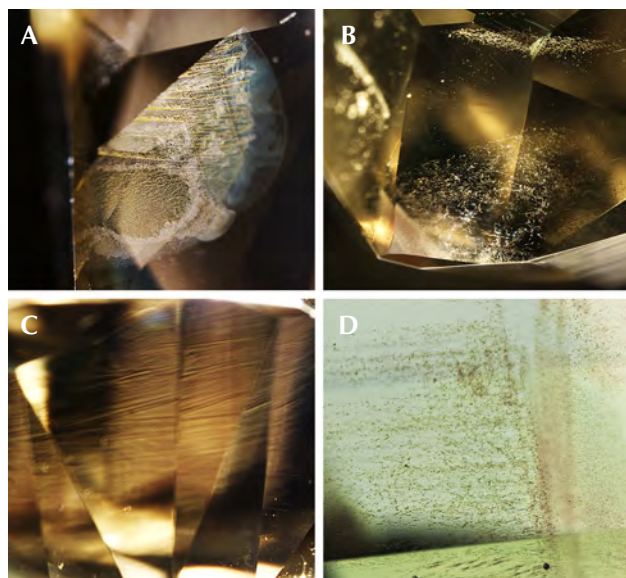
Figure 17. Inclusions in sapphires from Gombe: healed fissures with hazy edges (A), irregular particles and short needles (B), wavy graining (C), and flake-like particles (D). Photomicrographs in darkfield illumination (A–C) and diffused brightfield illumination (D) by Shunsuke Nagai. Fields of view 1.95 mm (A), 2.15 mm (B), 2.80 mm (C), and 2.80 mm (D).
