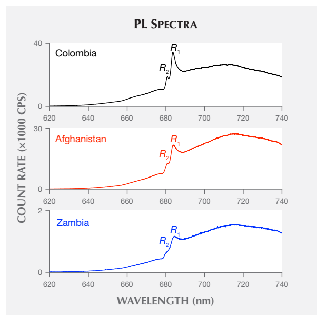
Figure 3. Photoluminescence (PL) spectra of emerald samples from the selected countries of origin were collected with the polarization axis of the excitation laser light aligned perpendicular to the crystal's c -axis. The black trace is from the Colombian sample shown in figure 1, the red trace from the Afghan sample, and the blue trace from the Zambian sample.
