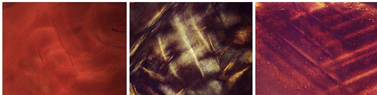
Figure 9. Grain boundaries as observed in transmitted light (left) are related to internal stress, which is best seen under crossed polarizers (center). Glide planes (Plato striations) are visible at the rim of the sample under identical illumination (right). Field of view 1.0 \times 0.75 mm (left and center) and 1.5 \times 1.1 mm (right). Photomicrographs by H.-J. Bernhardt.
