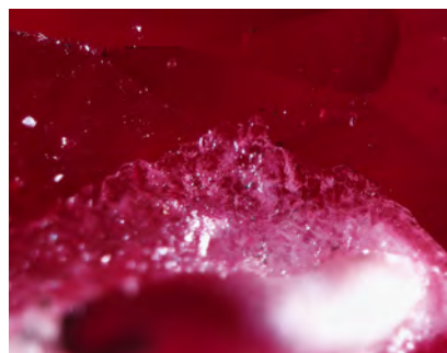
Figure 13. Synthetic overgrowth on the surface of a heated Burmese ruby. Field of view 1.50 mm.
