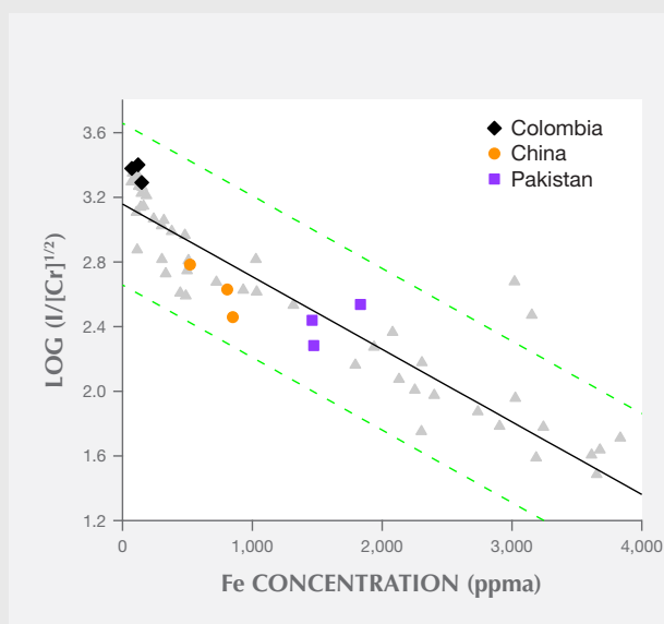
Figure B-1. Dividing PL count rates of each test sample's broadband peak emission I by the square root of its chromium concentration [Cr] , and taking the common logarithm, with the results plotted versus each test sample's iron concentration [Fe] . The black diamonds represent data from Colombian samples, the violet squares Pakistani samples, and the orange circles Chinese samples. The gray triangles reproduce the datasets presented in figure 13. The solid black trend line is a plot of the best-fit form of equation 2 to those datasets, and the dashed green lines form the boundaries of the equation's 95% confidence band.
