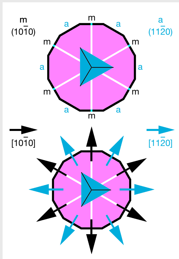
Figure A-1. Schematic representation of crystal faces (top) and crystallographic directions (bottom) in the crystal class of corundum, D_{3d} , with a view parallel to the c -axis. Symmetry elements depicted include the three-fold axis seen in the center and the mirror planes represented by white lines (two-fold axes are not given for simplicity). The first-order hexagonal prism \{10\bar{1}0\} is indicated by the symbol m and the second-order hexagonal prism faces a are parallel to mirror planes and parallel to the \langle 10\bar{1}0 \rangle directions.
