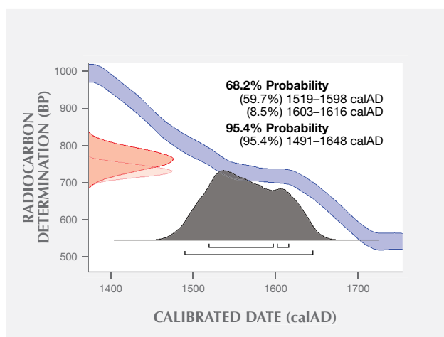
Figure 12. The University of Tokyo's radiocarbon dating results (both uncalibrated and calibrated ^{14}\text{C} age) of the shell powder from the same blister pearl sample.
