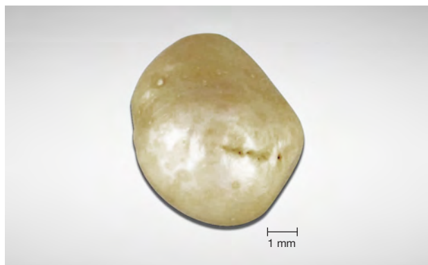
Figure 5. A small natural pearl used in an AMS experiment for this study. Photo by Masumi Saito.
