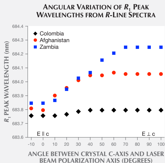
Figure A-2. The angular variation of R_1 peak wavelengths extracted from R-line spectra of emerald crystals from the three geographic origins.
