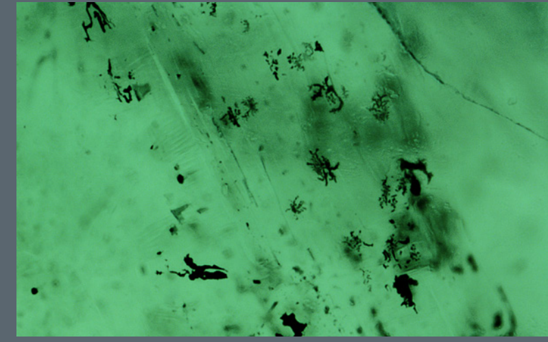
Skeletal platy crystals of ilmenite are scattered throughout this Zambian emerald. Field of view 1.91 mm.
