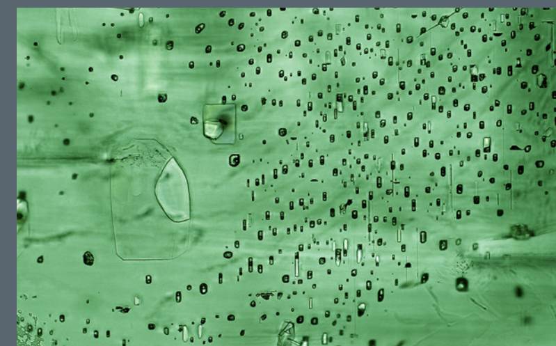
Blocky three-phase inclusions are crystallographically aligned in this Brazilian emerald. Field of view 1.42 mm.
