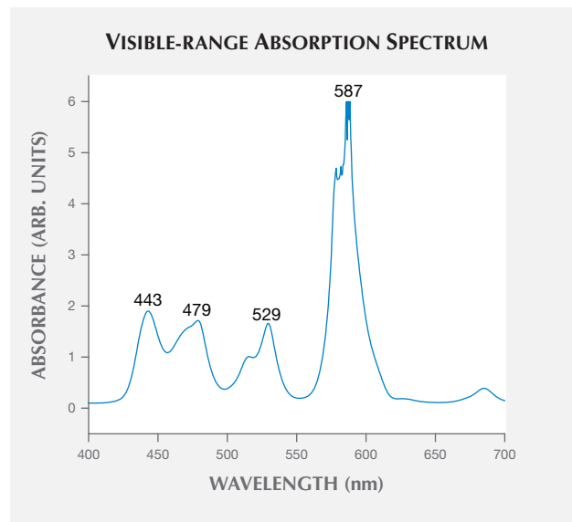
Figure 16. The visible absorption spectrum of the unmounted pear-shaped sample shows four absorption bands at 443, 479, 529, and 587 nm. The peak at 587 nm is associated with Nd 3+ , while the bands at 443, 479, and 529 nm are attributed to Pr 3+ .
