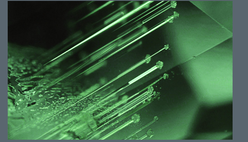
Nail-head spicules, as seen in this Regency hydrothermal synthetic emerald, are indicative of synthetic origin. Field of view 1.42 mm.
