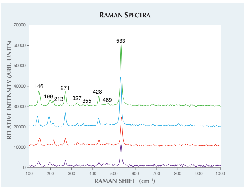
Figure 4. Raman spectra of four inclusions corresponding to coesite with high remnant pressure inside each inclusion. Spectra have been vertically offset for clarity.
