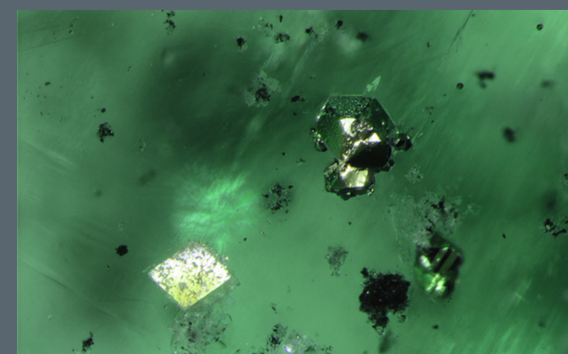
An inclusion suite often seen in Colombian emeralds consists of carbonates, pyrite, and fragments of black shale. Field of view 2.53 mm.
