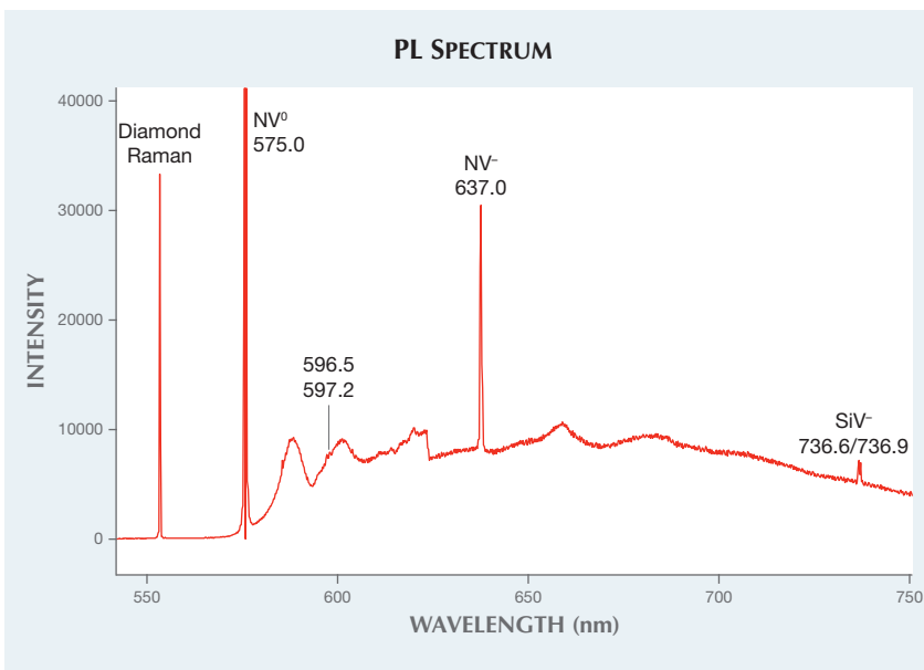
Figure 13. The photoluminescence spectrum acquired with 514 nm laser excitation revealed strong emissions from NV centers in addition to emissions from SiV - . Emissions at 596/597 nm indicated that this synthetic diamond was not annealed after growth.
