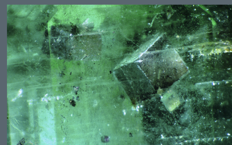
Several rhombohedral magnesite crystals are present in this emerald from Santa Terezinha de Goiás, Brazil. Field of view 8.68 mm.
