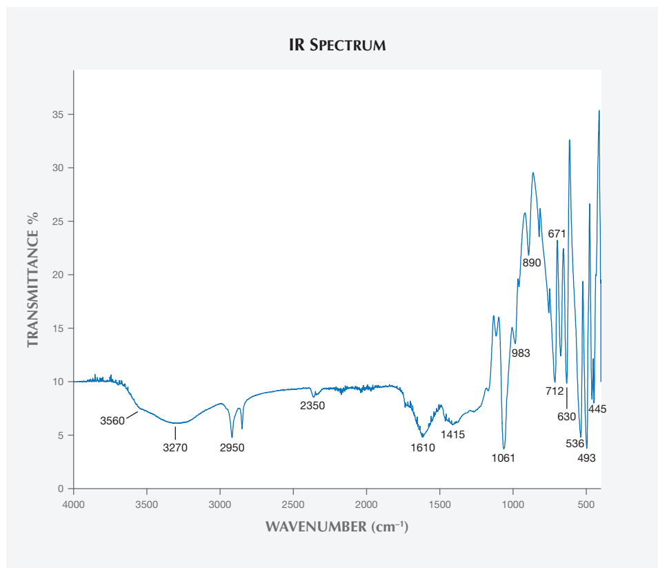
Figure 6. The infrared spectrum of powdered danburite from Luc Yen shows a broad band centered at 3270 cm^{-1} and a weak band at 3560 cm^{-1} , both of which are related to stretching vibrations of the OH^{-} group.
